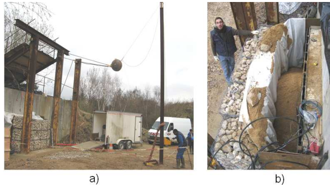
Figure.2. Overview of the experimental device (a) and the impacted structure during the implementation (b).
