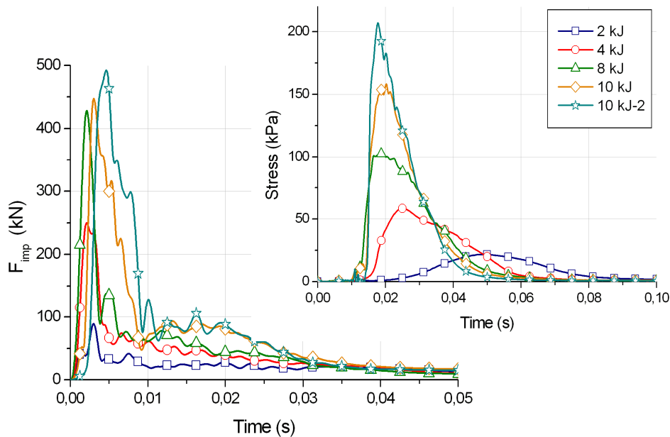
Figure.4. (left) Impact force F_{imp} of the projectile vs. Time for each impact energy; (right) Stress measured at the support vs. Time for each impact energy.
